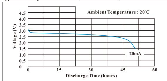
Typical Discharge Characteristics (20mA Continuous)
